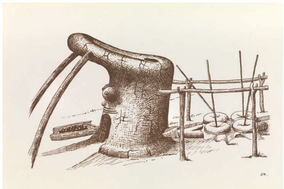
7 Diagram of Chokwe furnace, Kaparandanda, Alto Zambezi, Angola, rendered by José Redinha, 1953.
